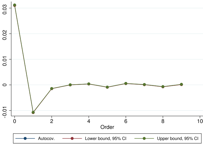
FIGURE OA.19.—Autocovariances of return residuals. Notes: The figure shows the sequence of estimated \text{cov}(\hat{\Delta}\hat{u}_{i(g)t}, \hat{\Delta}\hat{u}_{i(g)t-j}) for j = 0, \dots, 9 from the regression in Table 4, column (3), in the main text.
