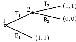
FIGURE 4.—Game tree from the discussion on admissibility.
