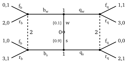
FIGURE 1.—Game tree from Example 2.1.
