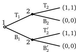
FIGURE 2.—Game tree from Example 3.4.
