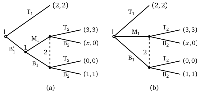
FIGURE 3.—Game trees from Example 4.1.
