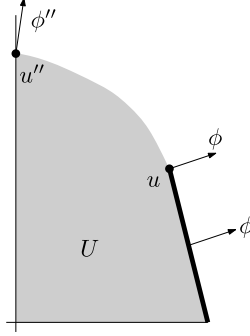
FIGURE E.1.—The maximal extreme point u is not exposed while U^p = U^{++} .
