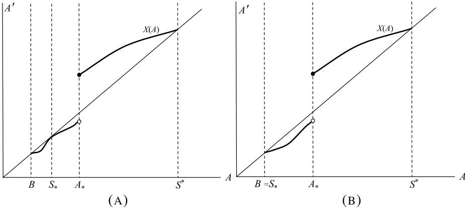
FIGURE A.1.—The two sustainable assets S_* and S^* . (A) S_* > B . (B) S_* = B .
