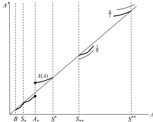
FIGURE A.2.—Outline of the proof starting from Lemma 27.
