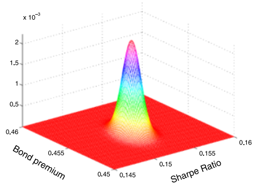
(c) Joint distribution f(\omega)
