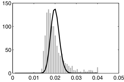
FIGURE 1. Implied unconstrained probability density function g(\omega|\bar{X}) and its approximation by a Gamma distribution (solid line).
