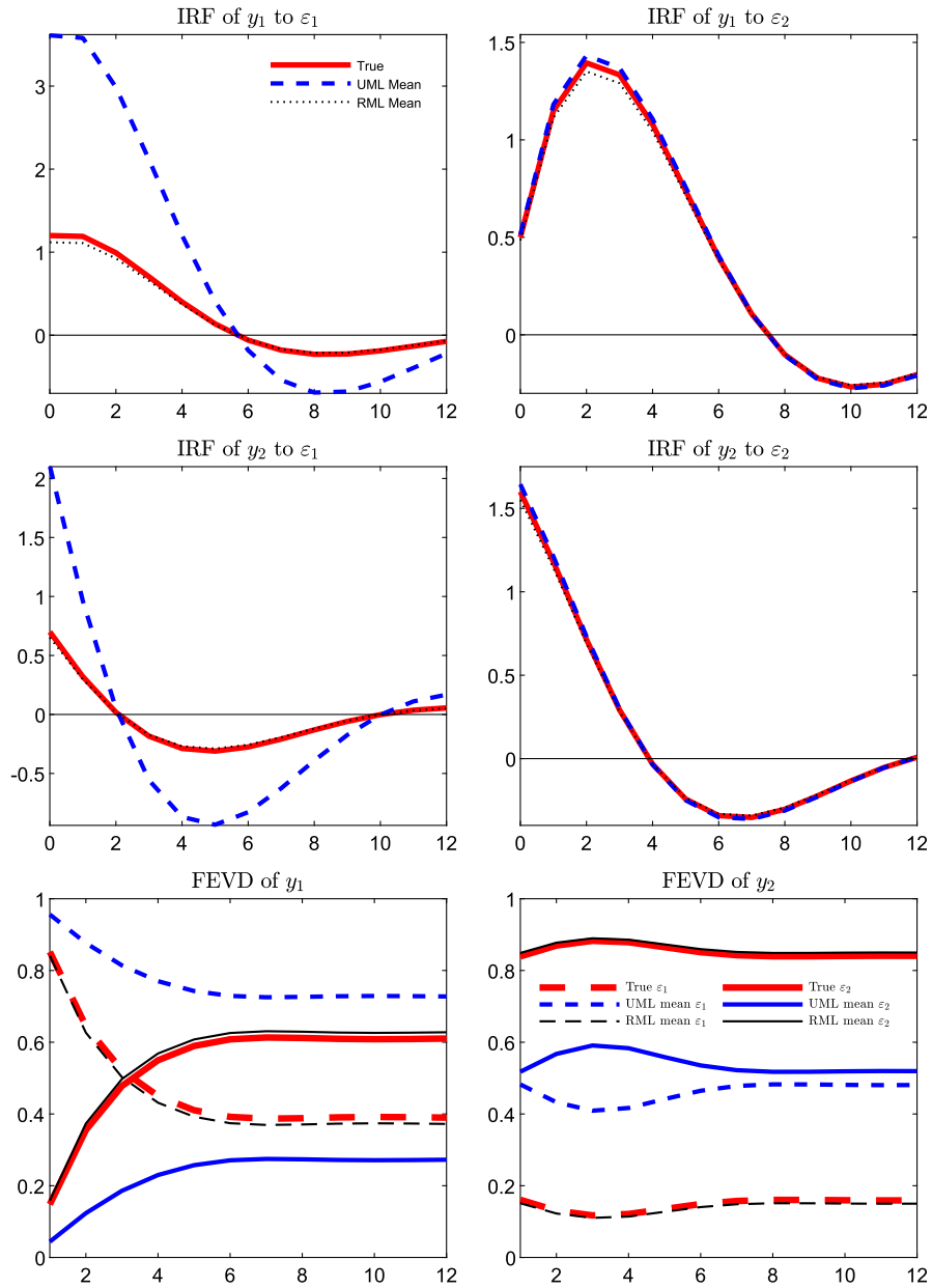
FIGURE 1. IRF and FEVD. DGP: Independent DLSMN _{(\delta_1, \kappa_1, \lambda_1)=(0,0.52,0.06), (\delta_2, \kappa_2, \lambda_2)=(0.3,0.2,0.2)} .
